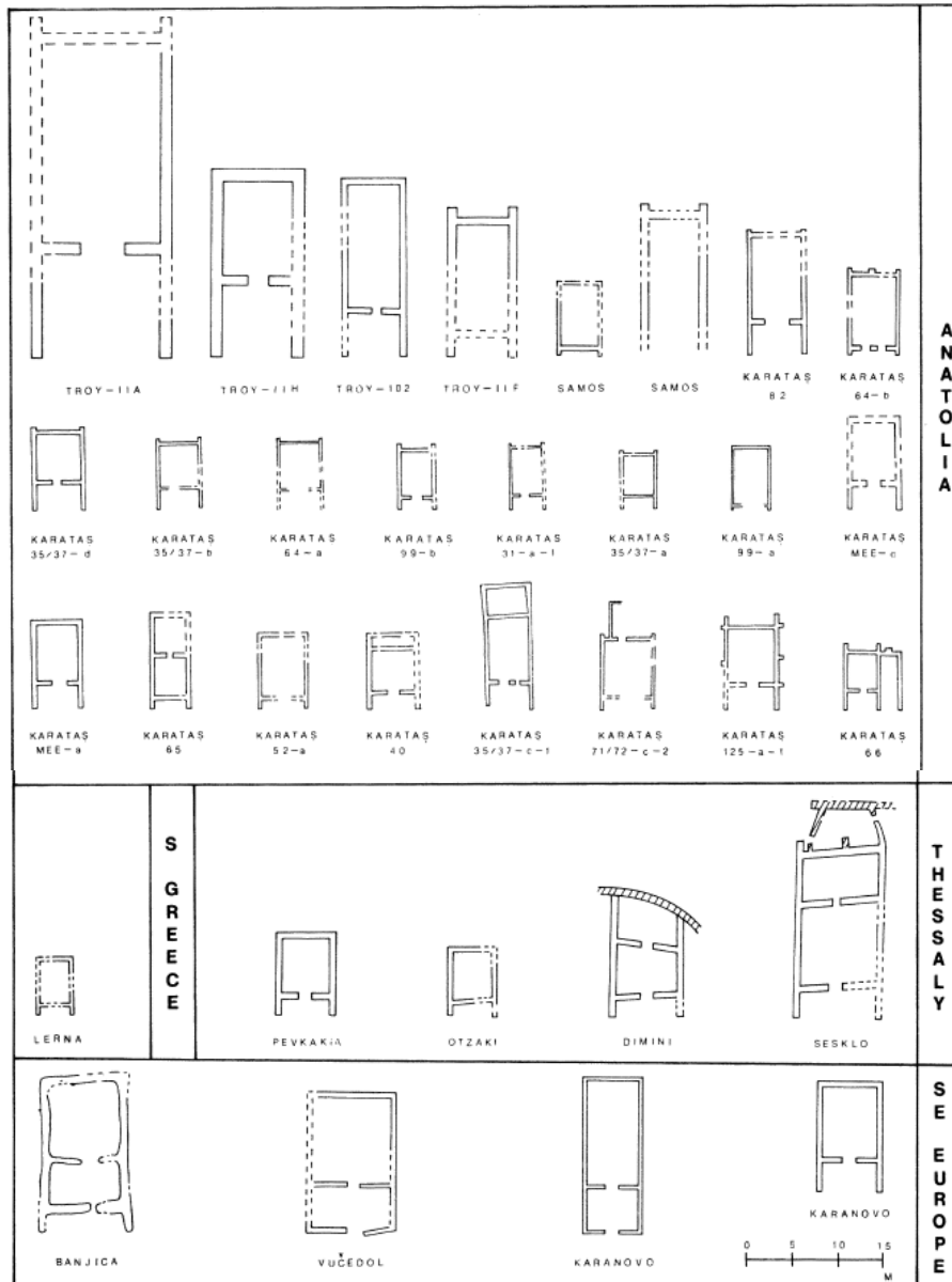
ILL. 2. Comparative chart of megara (drawn approximately to the same scale)
